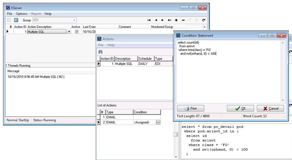
The EDI monitor displays recent and current activity in high volume environments, supporting easy access to messaging and quick responses to issues requiring attention.
